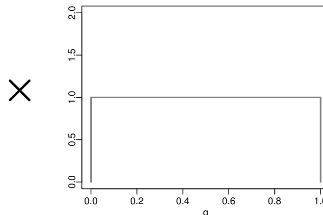
q の事前分布 (prior)
